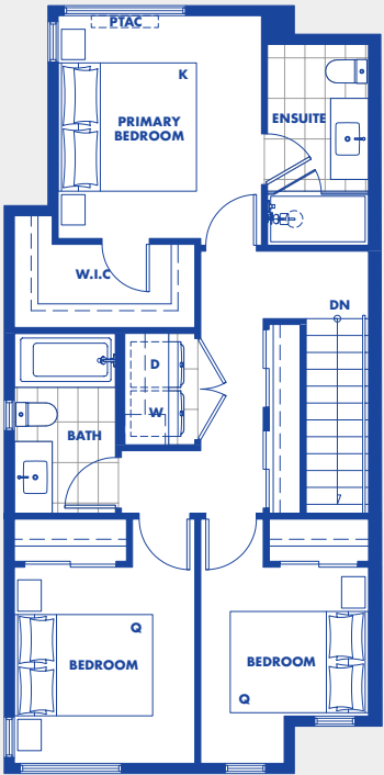
UPPER FLOOR
