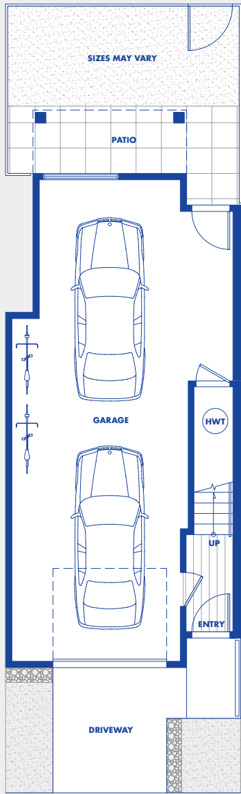
LOWER FLOOR
