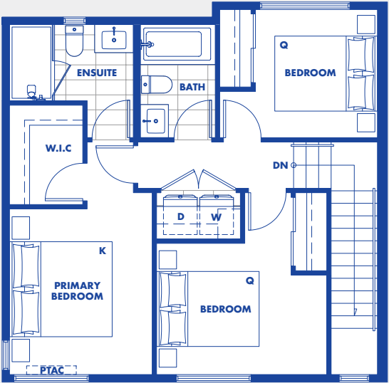
UPPER FLOOR
