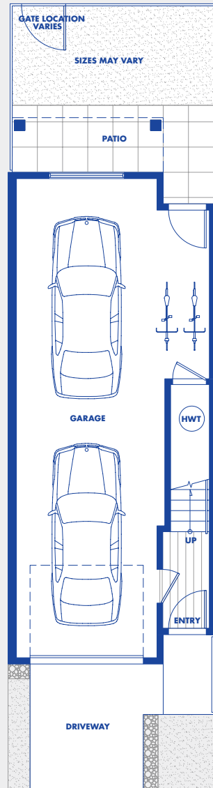
LOWER FLOOR
